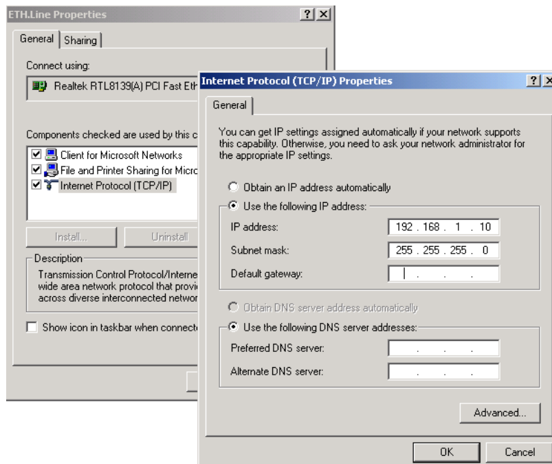
Picture 1 – PC network configuration
